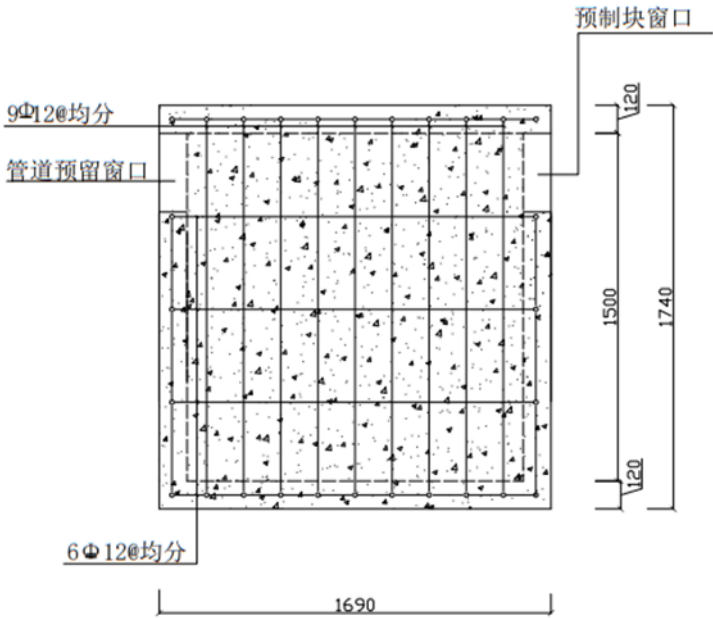
1450*840*1500 (A-立面图配筋图)
