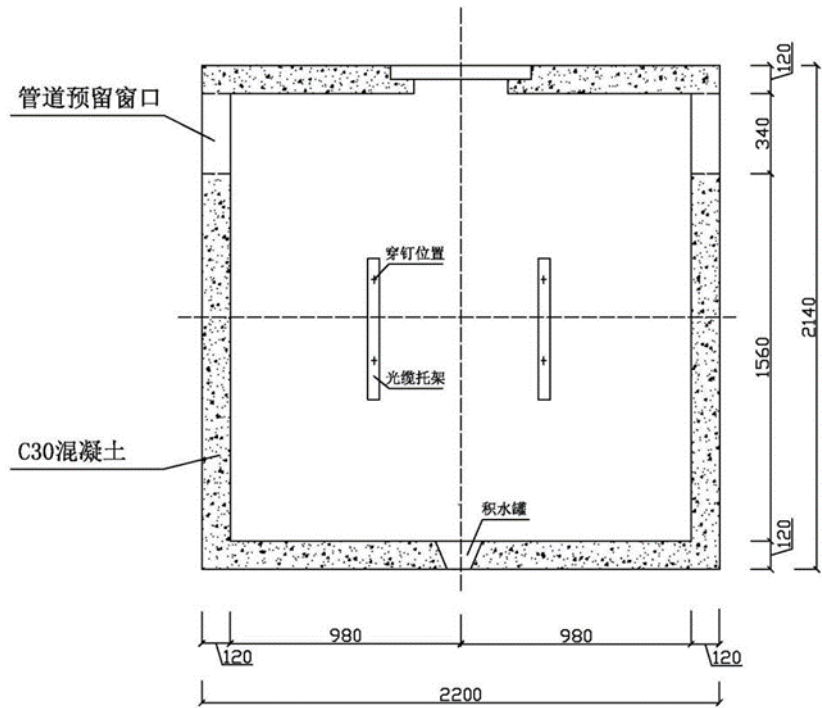
1960*1410*1900 (A-立面图)
